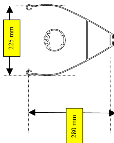
Section de bôme MK 2R
